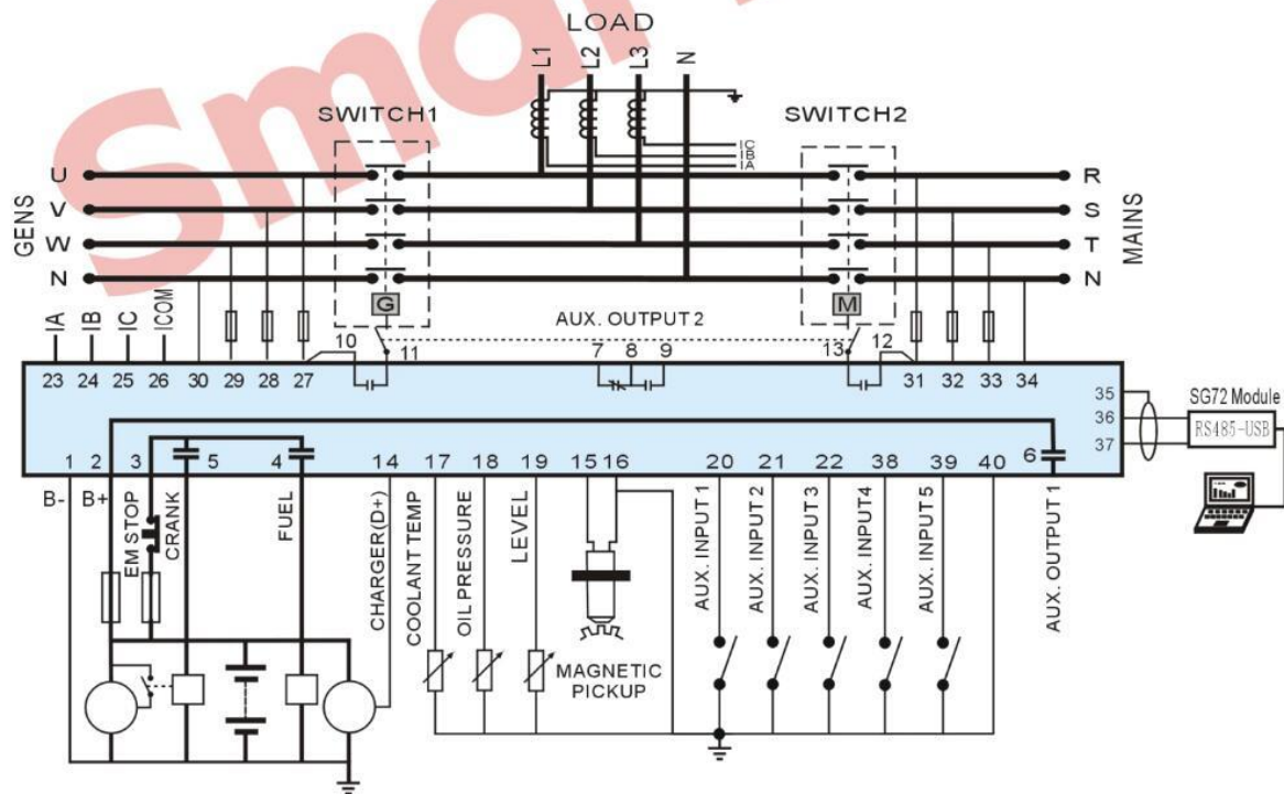
HGM6120UC Typical Application Diagram
